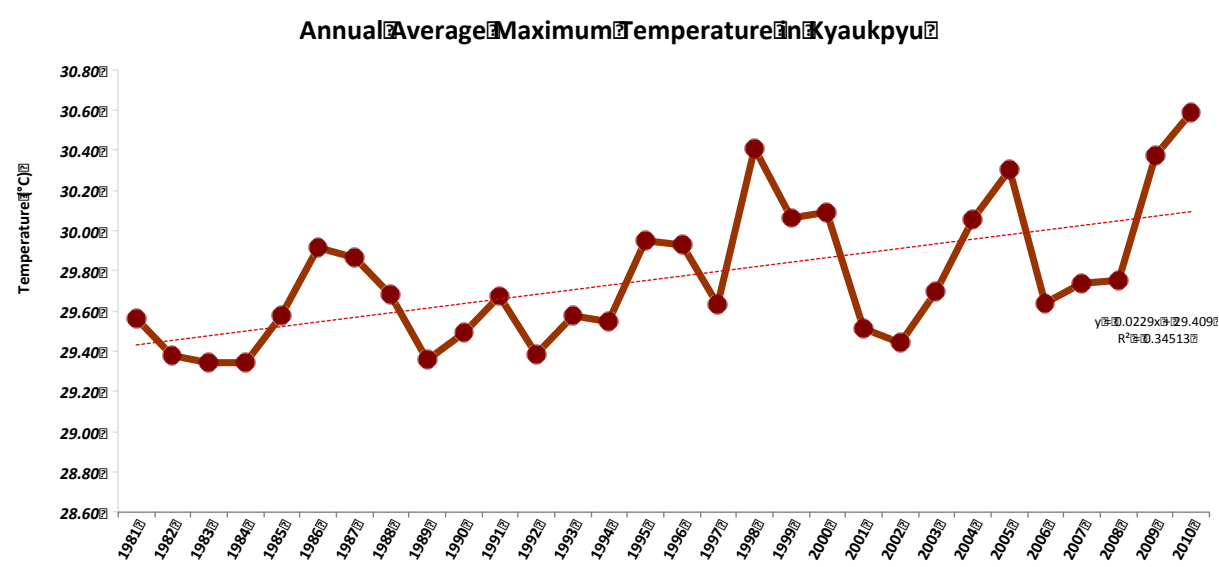
Figure 21. Annual average maximum temperature, in Kyaukpyu, from 1981-2010 showing inter-annual variability and increasing trend.
