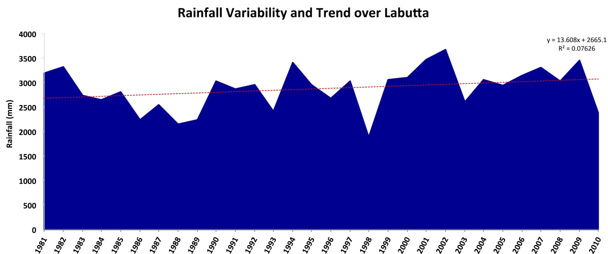
Figure 46. Rainfall variability and trend, over Labutta, based on observed data from 1981-2010.
