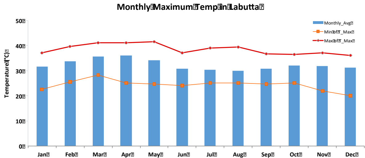
Figure 44. The blue bars show the monthly average maximum temperature in Labutta, based on data from 1981-2010. The red marked lines indicate the highest observed maximum temperature in particular months; the orange marked lines identify the lowest observed maximum temperature.
