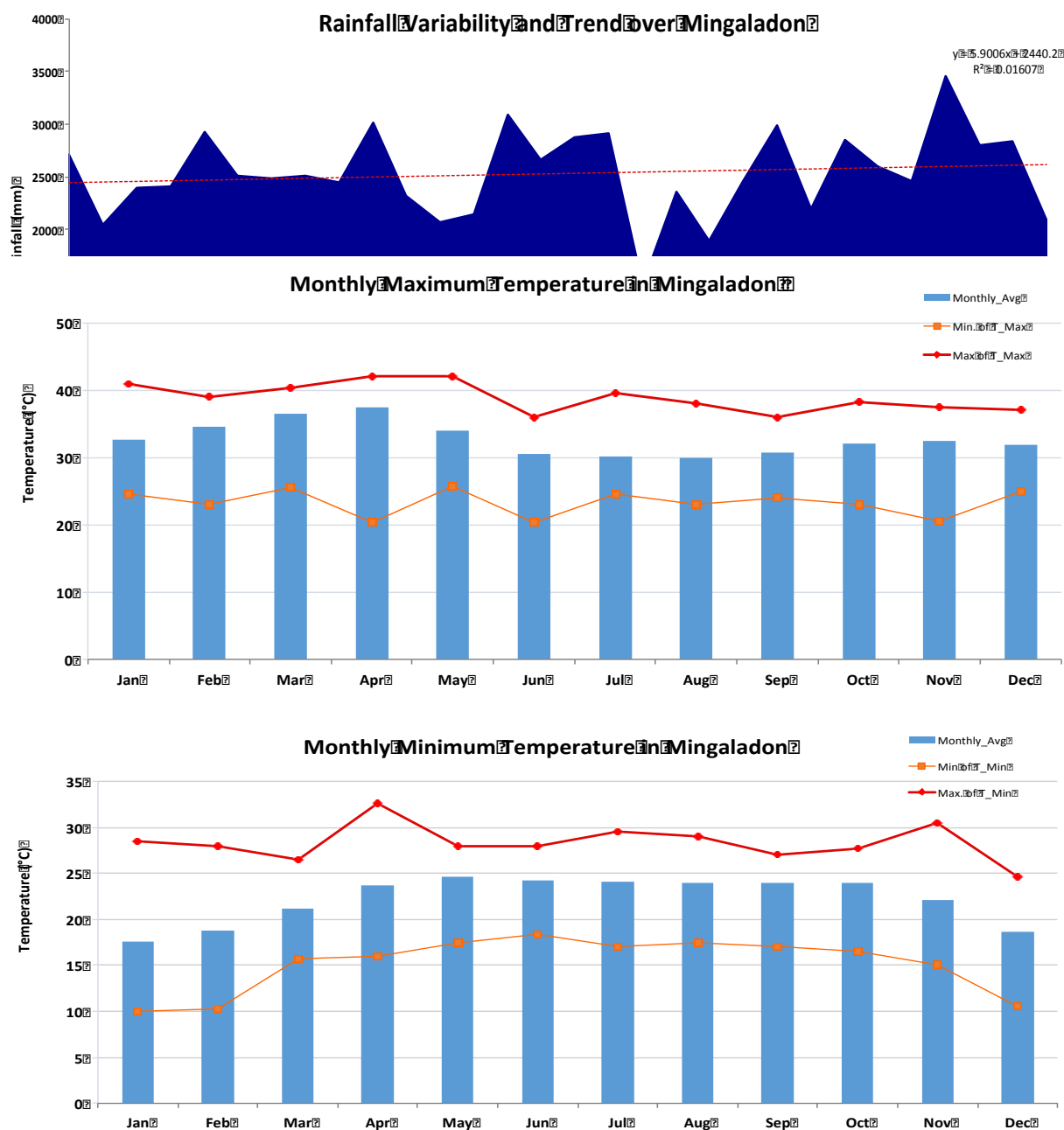
Figure 53. Monthly maximum (above) and minimum (below) temperature (in blue bars); the marked red line shows the highest maximum and minimum temperature recorded in various months; while the orange marked line indicates the lowest maximum and minimum temperatures in various months.
