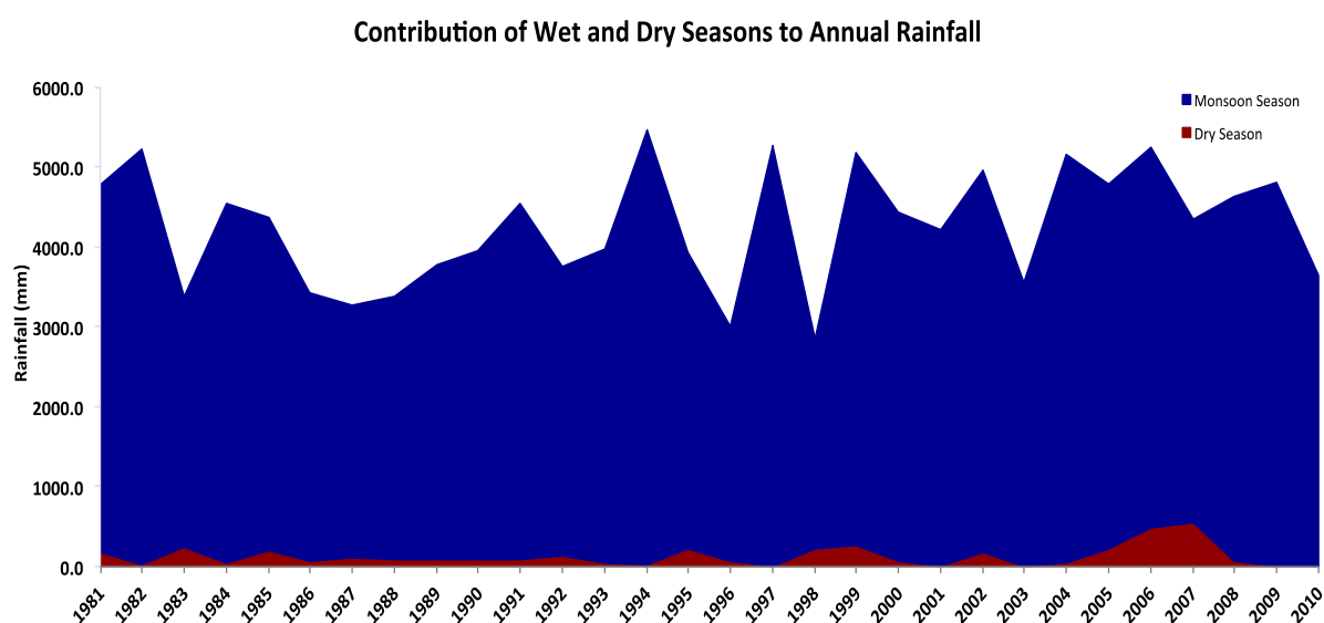
Figure 38. Wet and dry seasons contribution to annual rainfall in Hpa-An, from 1981-2010.
