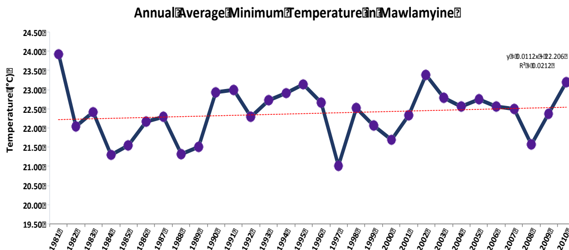
Figure 32. Annual average minimum temperature in Mawlamyine. On the average, the warmest nights were recorded in 1981; the coolest nights were in 1997.
