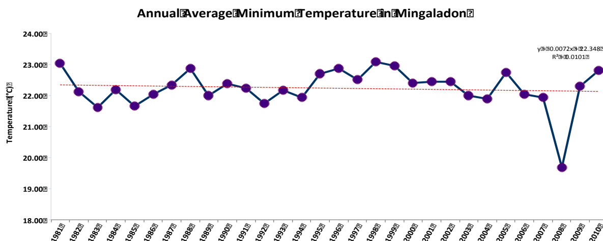
Figure 57. Annual average minimum temperature in Mingaladon. The warmest nights, on average, were in 1998, the warmest nighttime temperature was in 1 April 1998 (32.6°C, the only nighttime exceeding 30°C; also the warmest night within 30 years). 252 nights exceeded the average minimum temperature; of these, 85 nights exceeded 25°C.
