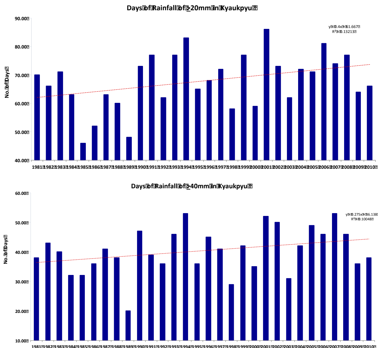
Figure 20. Heavy rainfall events, of \geq 20\text{mm} and \geq 40\text{mm} (above and below, respectively) manifesting an increasing trend.
