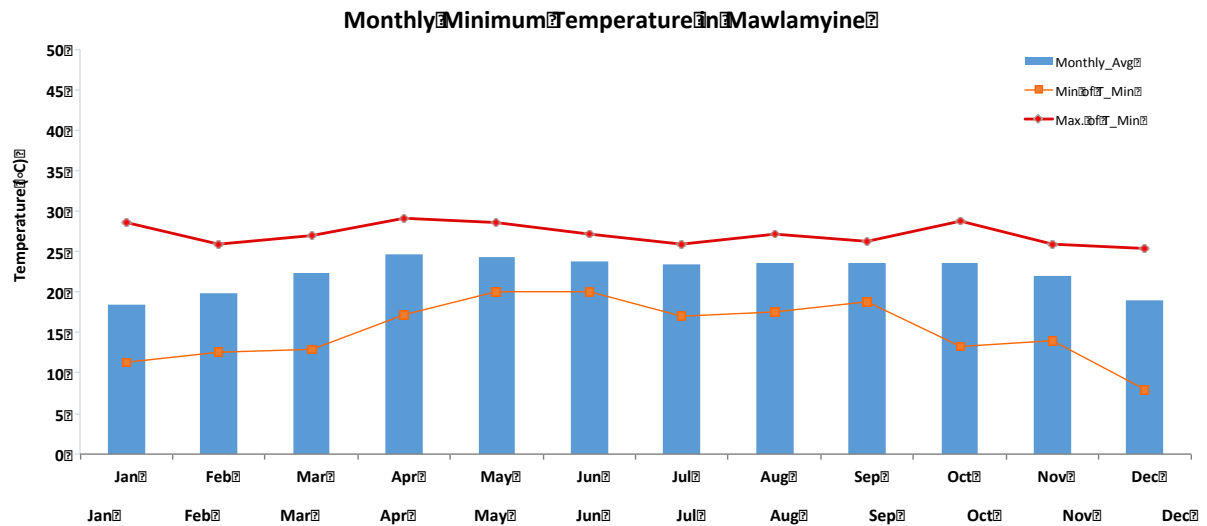
Figure 26. Average monthly minimum temperature in Mawlamyine, in blue bars; the red marked lines indicate the highest recorded minimum temperature; the orange marked lines provide the lowest observed minimum temperatures. The change in rainfall being lower than the first half of the year, as with many other areas in the country influenced by the Southwest Monsoon
