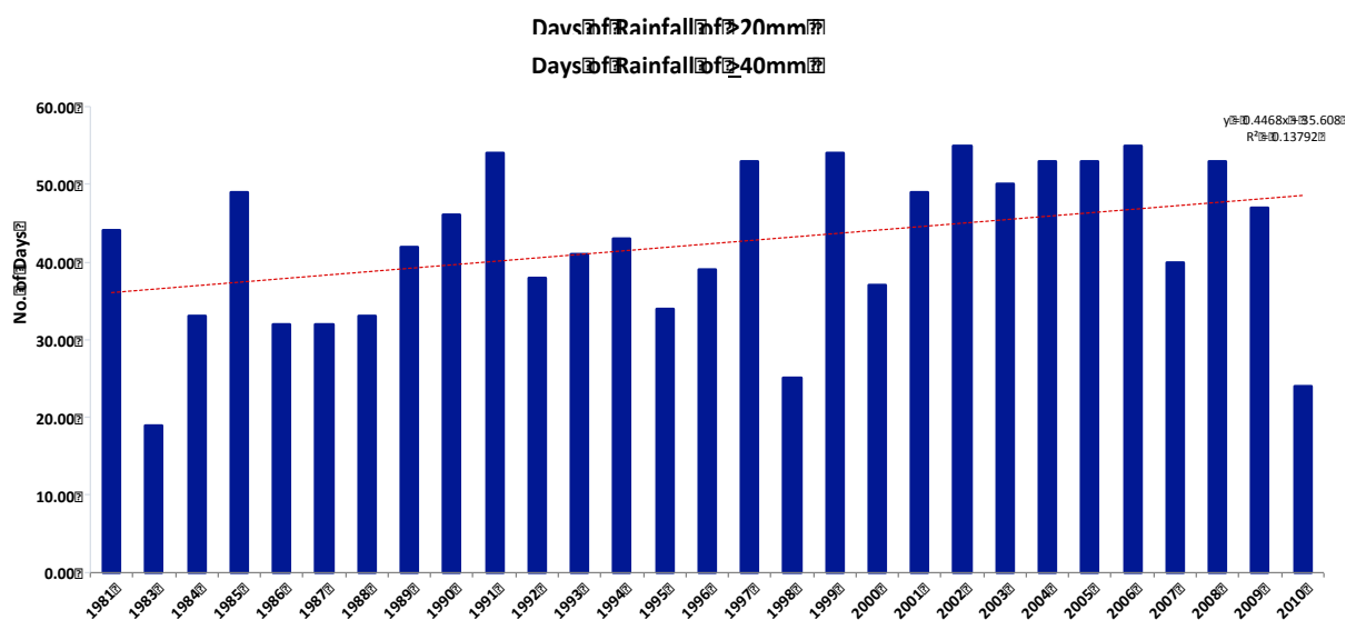
Figure 30. Heavy rainfall events \geq 40\text{mm} manifest an increasing trend in Mawlamyine.
