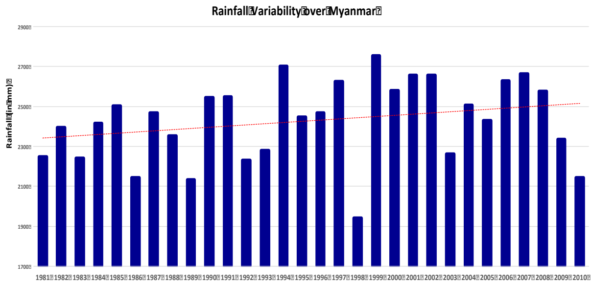
Figure 3. Inter-annual rainfall variability over Myanmar, from 1981-2010.
