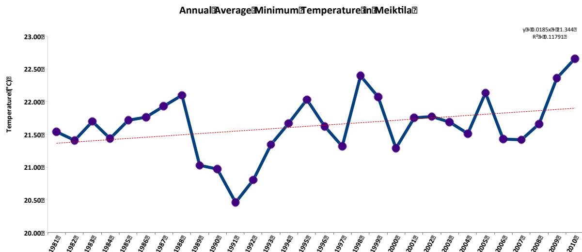
Figure 13. Variability in average nighttime temperature in Meiktila, from 1981-2010. Warmest nights were recorded in 2010; the coolest nights were in 1991.
