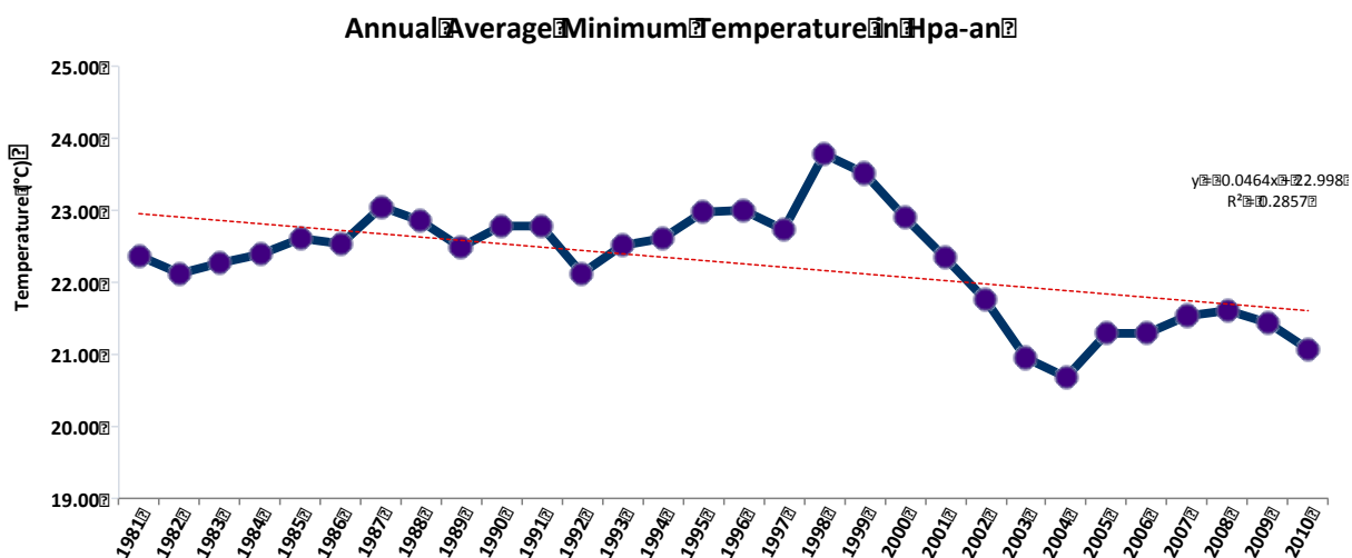
Figure 36. Annual average minimum temperature in Hpa-an, from 1981-2010. The warmest nights, on the average, were in 1998 and the coolest nights were in 2004.
