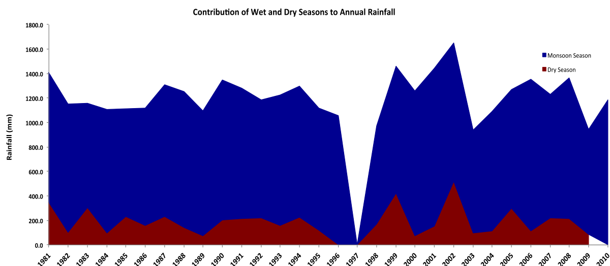
Figure 63. Wet and dry seasons contribution to annual rainfall in Kengtung. The data shows significant rainfall from months outside of the May to October period.
