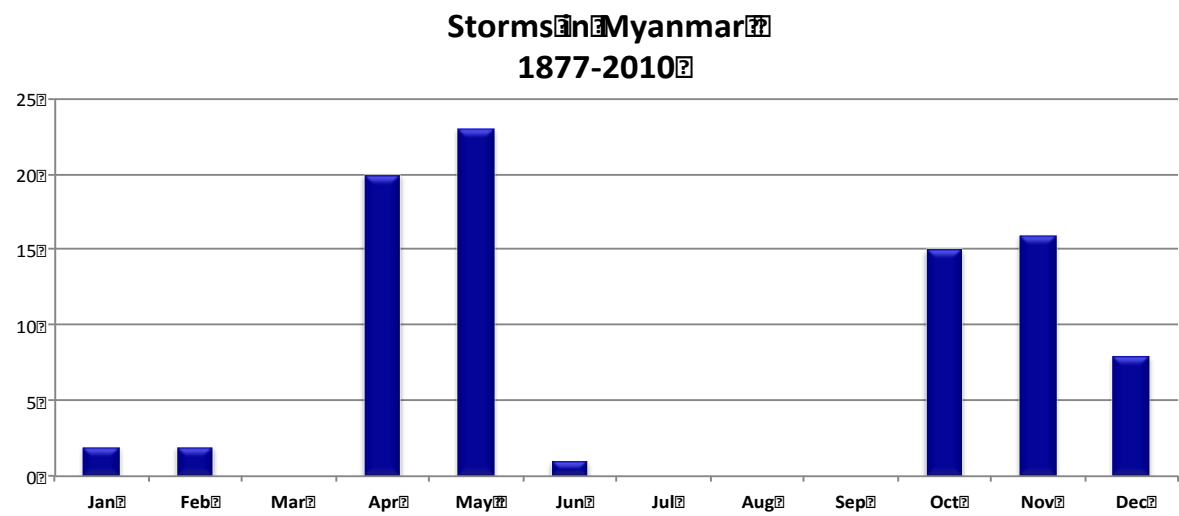
Figure 2. Storms that crossed Myanmar from 1877-2010.
