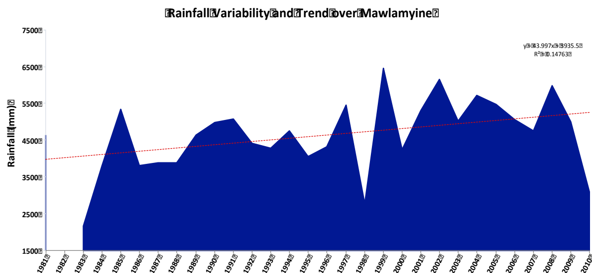
Figure 27. Rainfall variability and trend over Mawlamyine, from 1981-2010; data, for 1982, is not available.
