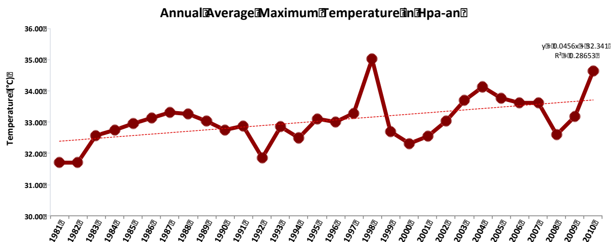
Figure 40. Variability and trend in annual average maximum temperature, in Hpa-An, from 1981-2010
