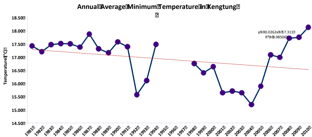
Figure 66. Annual average minimum temperature in Kengtung, from 1981-2010. The warmest nights, on the average, were in 2010; on the other hand, the coolest nights were in 2004. Temperature data, from 1995-1997, is unavailable.
